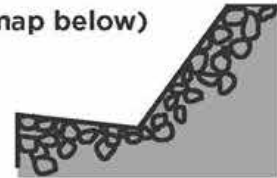
CATCHBENCH
